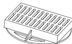
Rain water drain 400x60 mm full, plate max. Ø700mm outlet max. Ø360mm class C250÷D400
