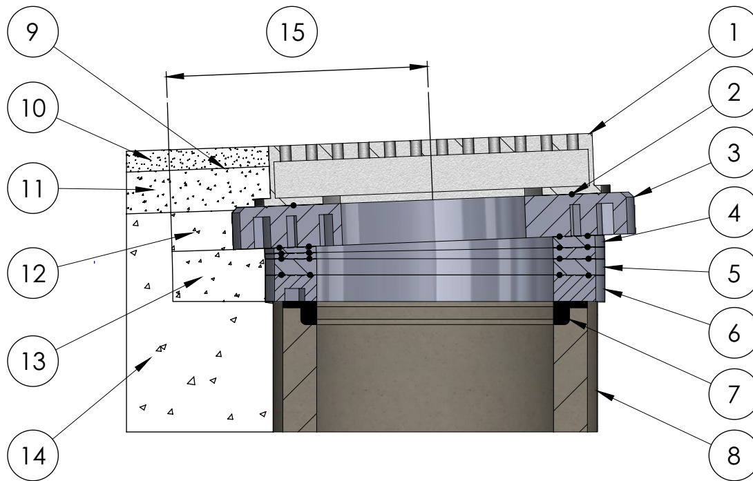
Diagram of a tight TVR T System surface finial of a sewage drain.
