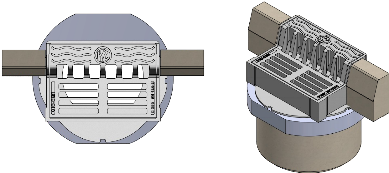
KZO WUKJC - H150 C250 roadway and kerb drain
