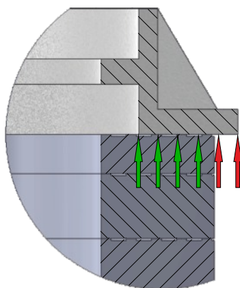
❗ Fig. 4. Incorrect selection of support, compensation, and well final elements. Lack of design integrity of final components and lack of support for the portion of manhole body.
