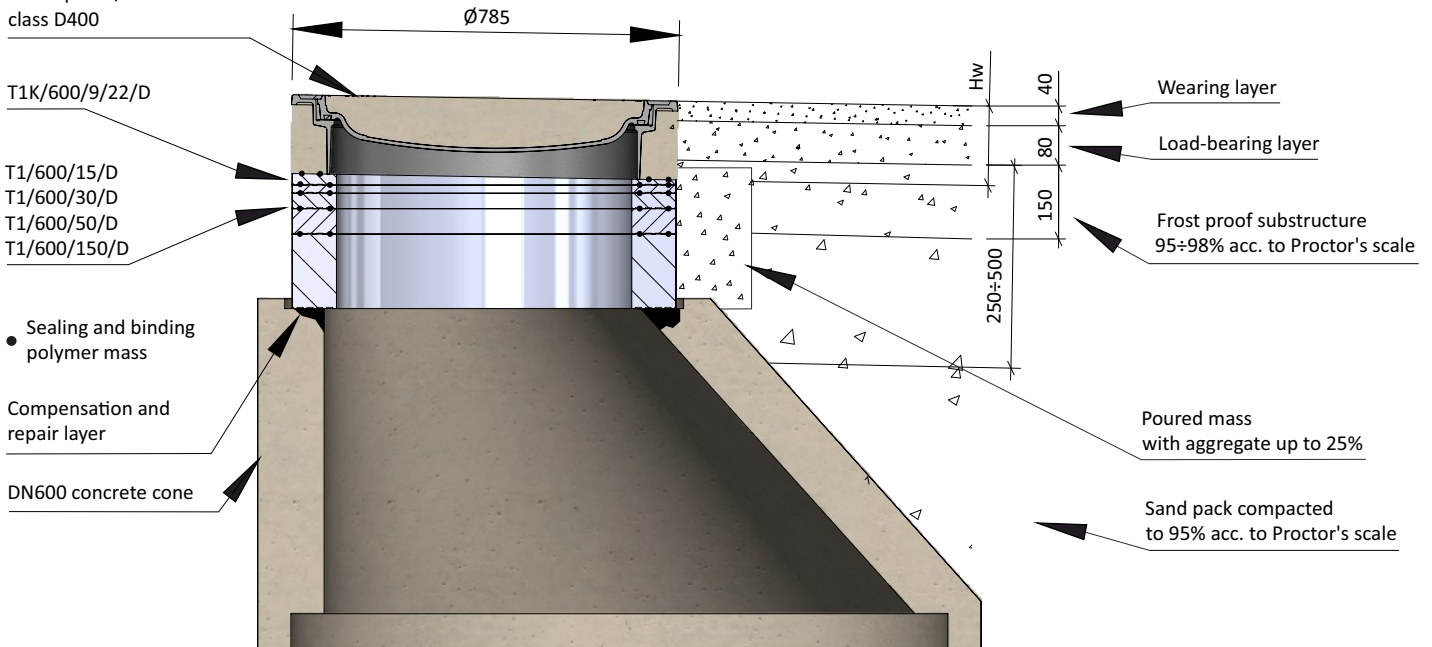
DN600 sewage manhole round plate Ø max. 785mm class D400
