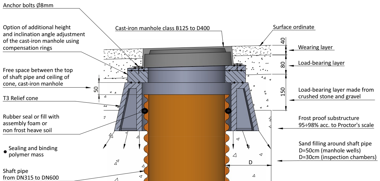
Fig. 7. Surface finial of plastic wells
