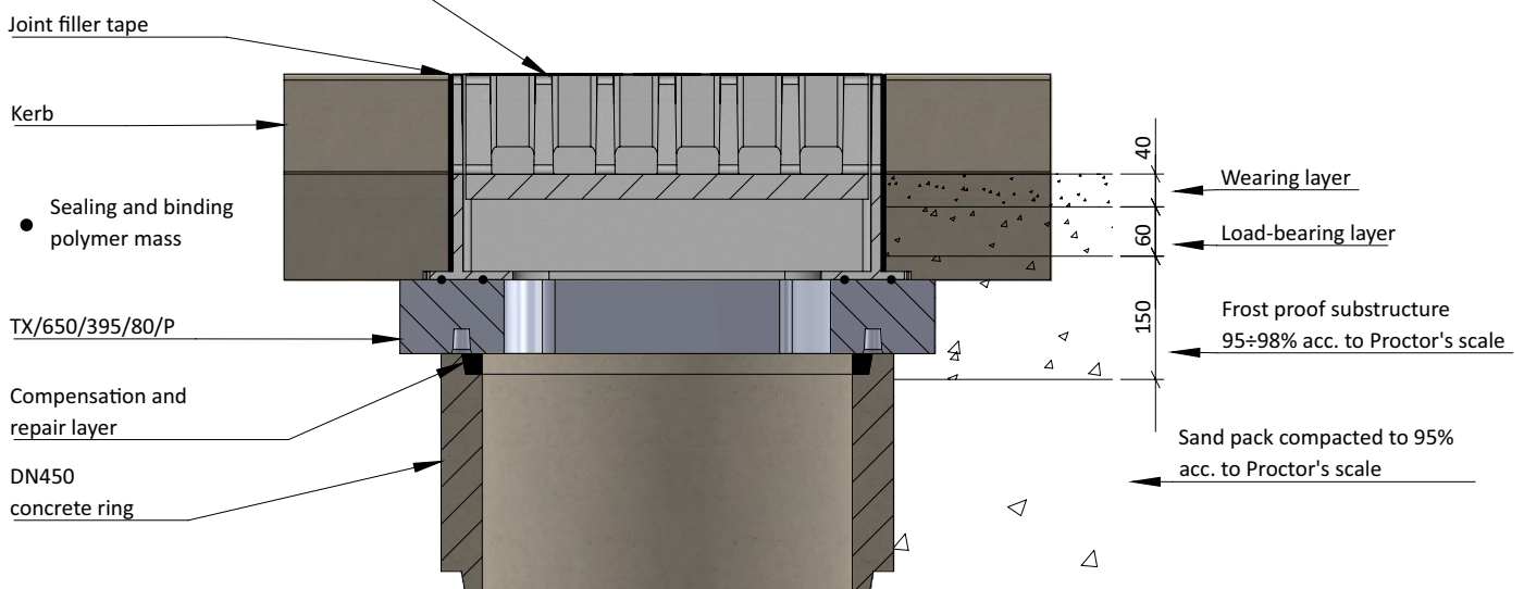
KZO WUKJC - H150 C250 roadway and kerb drain
